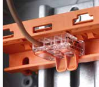
Terminal levers can also be operated without difficulty when assembled.
